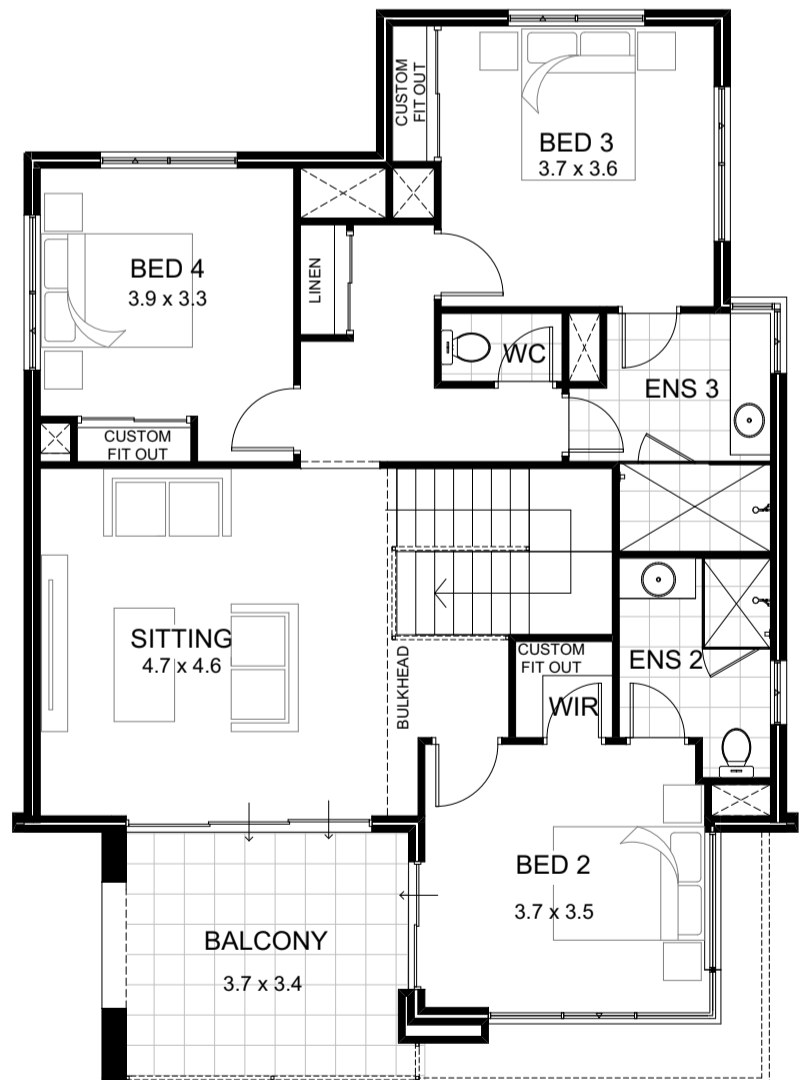
UPPER FLOOR
