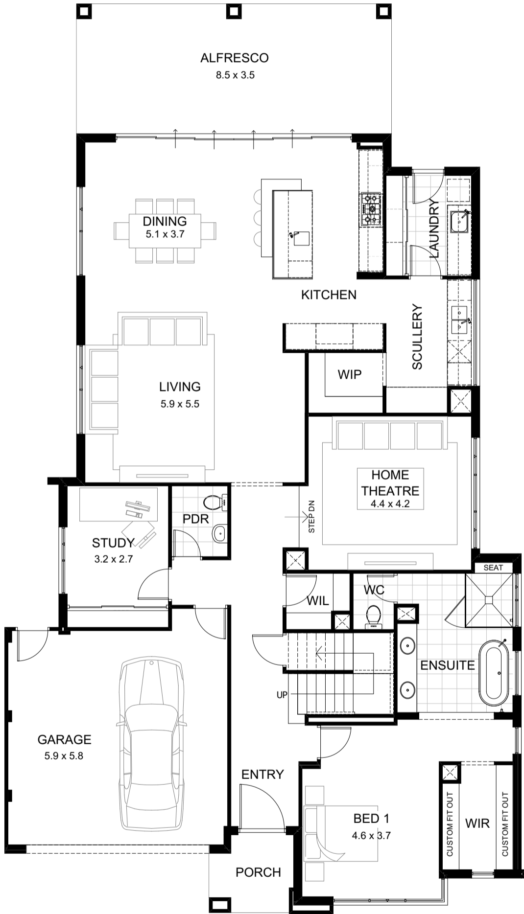
GROUND FLOOR
